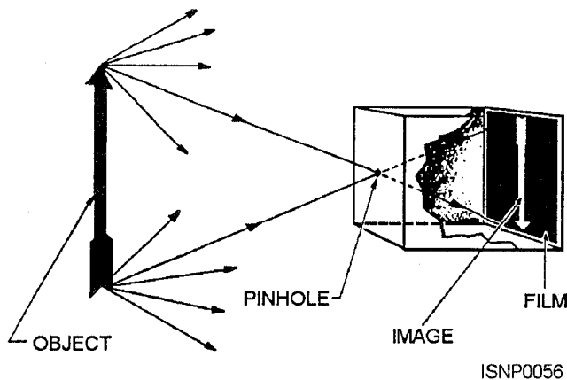
Figure 6-6.—Pinhole camera.
